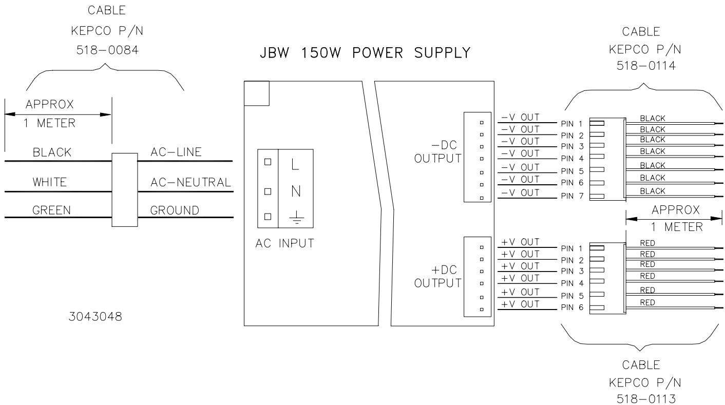
FIGURE 1. CABLE KIT INSTALLATION
